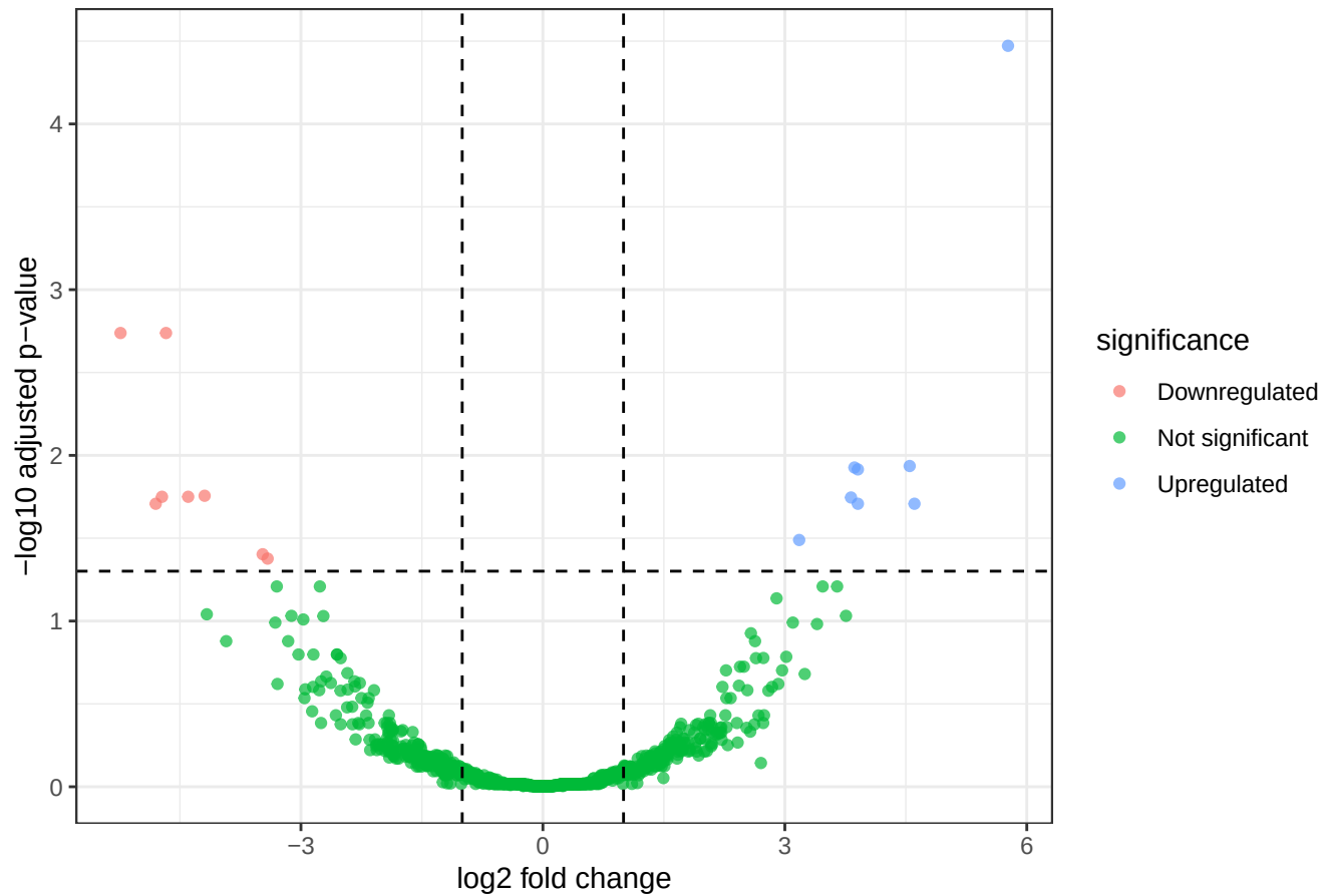
Volcano plot: treatment vs control
